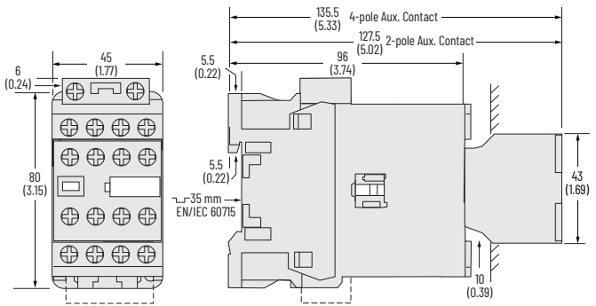
Figure 48 - 100-E26...100-E38 4-Pole Contactors with Standard Coils and Front-mounted Auxiliary Contact
